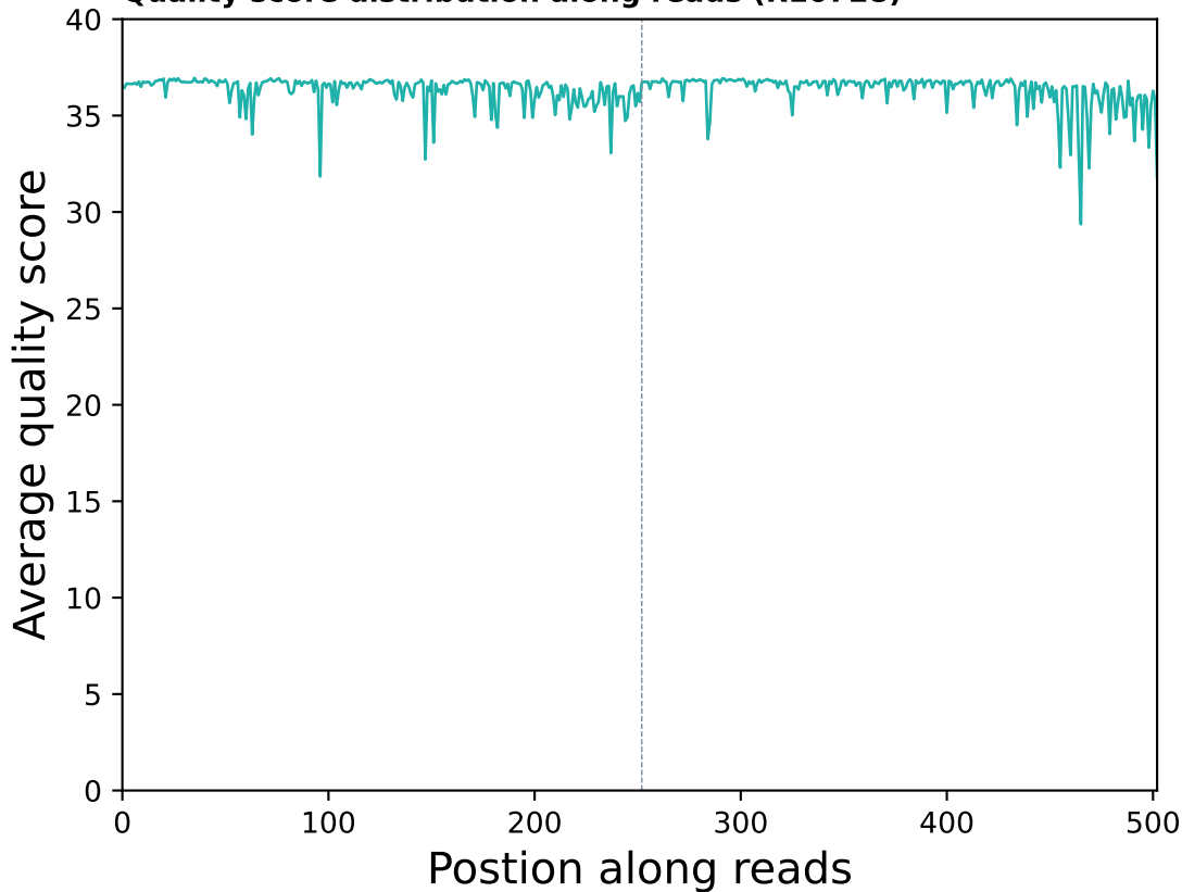
Quality score distribution along reads (R10728)
